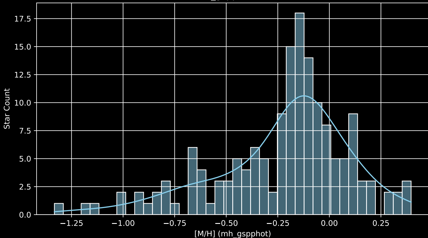
APOGEE DR17 Field: [K2_C2_348+16_btx [M/H] (mh_gspphot) (n= 159)
