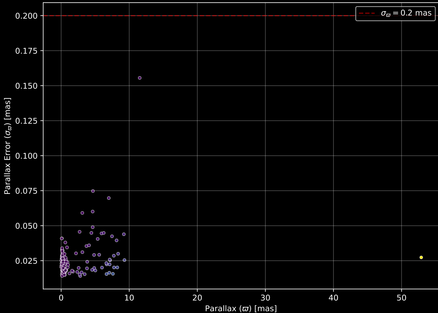
APOGEE DR17 Field: [K2_C2_348+16_btx] Parallax Quality (n= 159)
