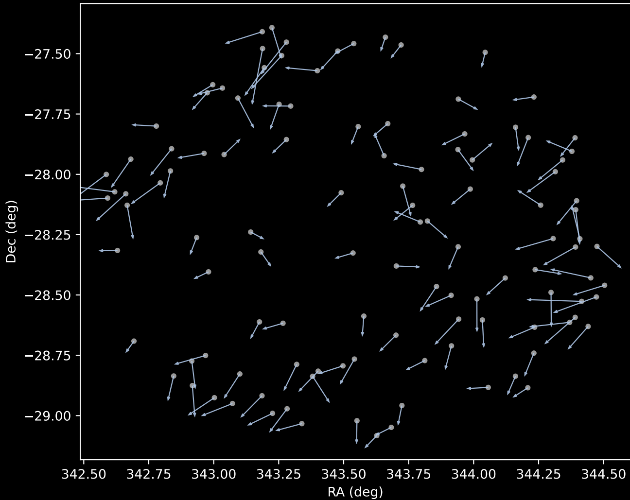
APOGEE DR17 Cluster 1 Proper Motion Vectors (n=114)
