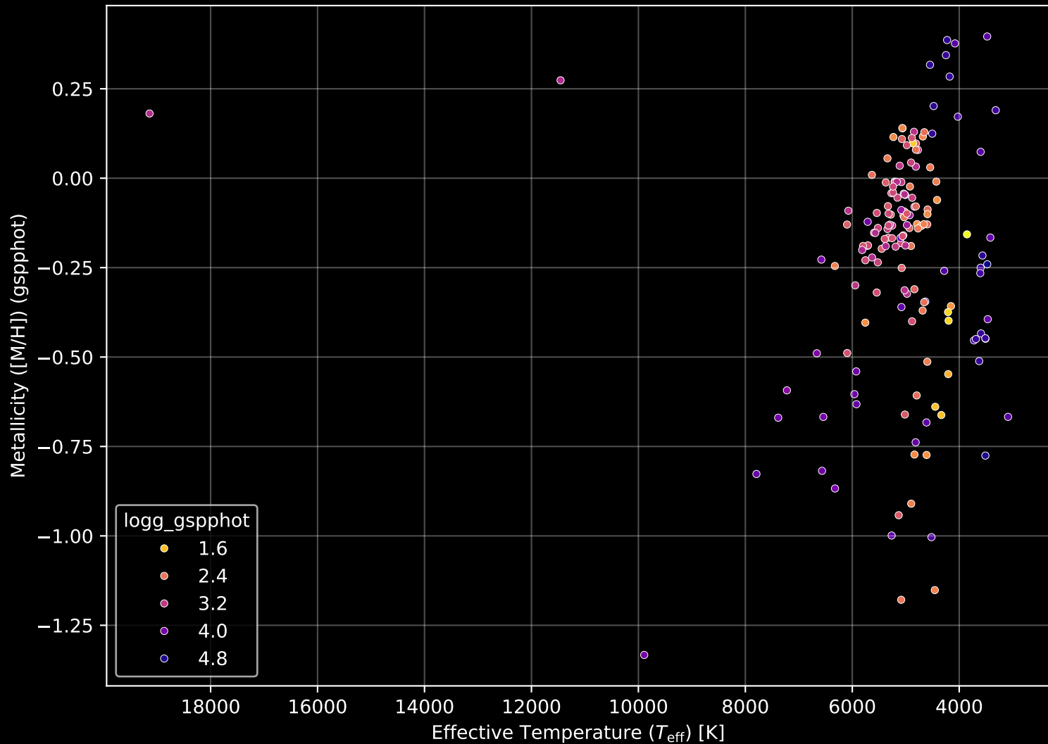
APOGEE DR17 Field: [K2_C2_348+16_btx] Stellar Population Parameters (n= 159)
