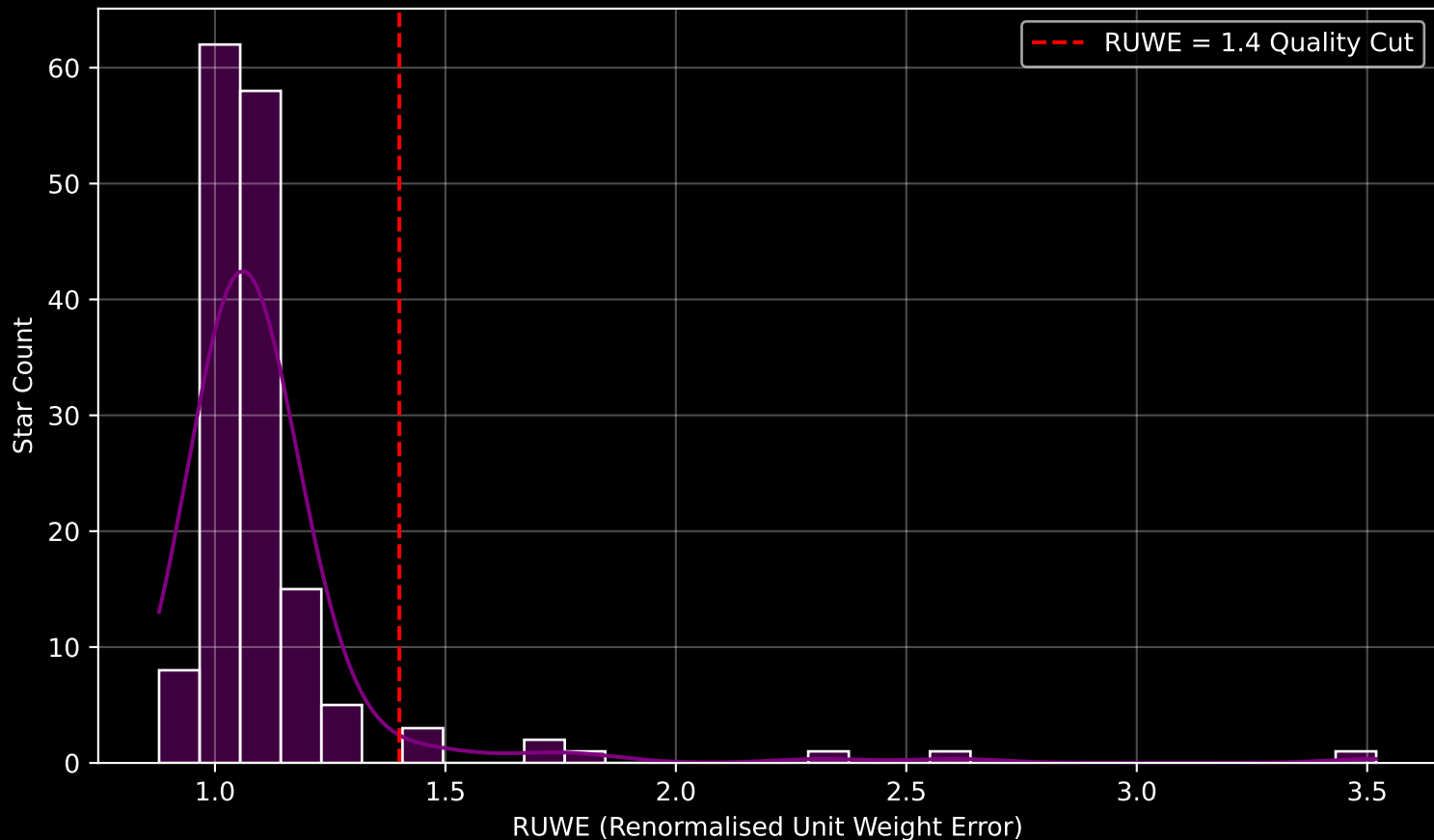
GAPOGEE DR17 Field [K2_C2_348+16_btx] RUWE Distribution (n= 157)
