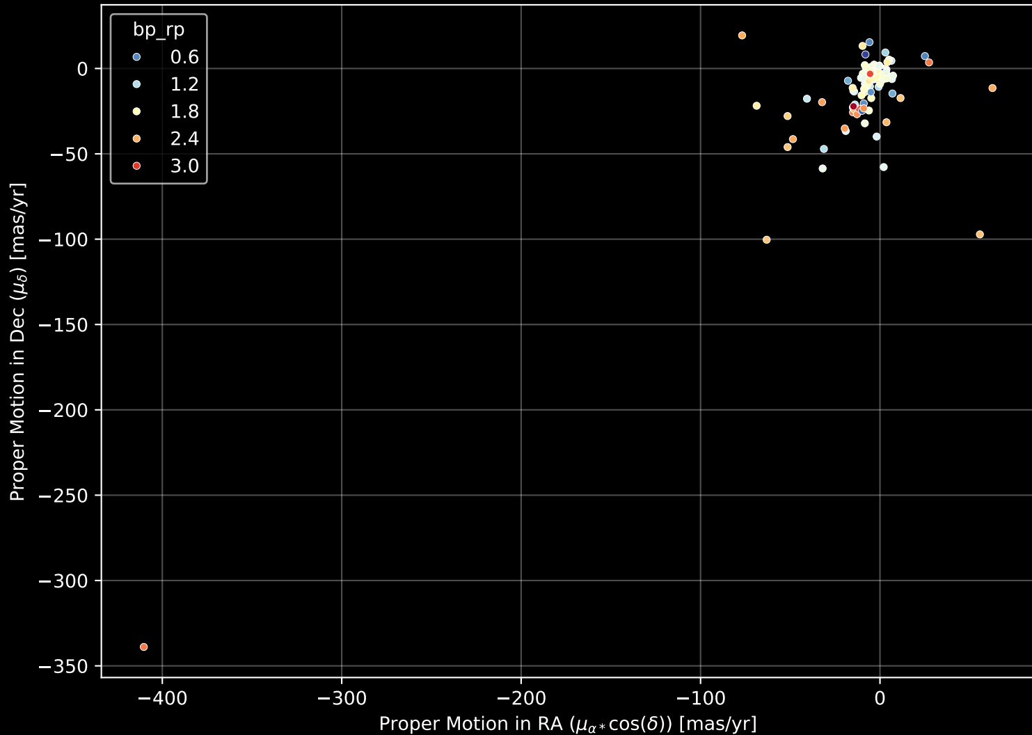
APOGEE DR17 Field: [K2_C2_348+16_btx] Proper Motion Diagram (n= 159)
