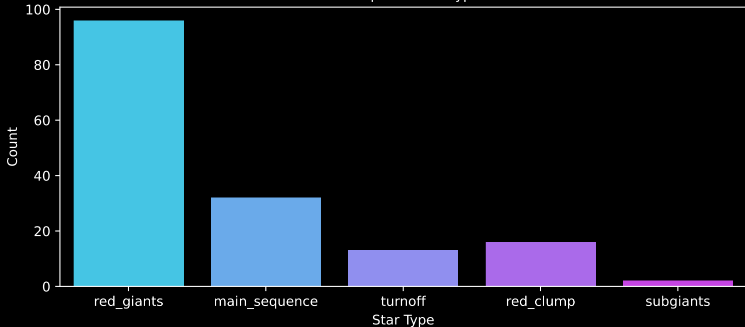
APOGEE DR17 Field: [K2_C2_348+16_btx] Count plot of Star Type
